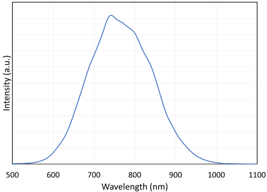
Figure 1: Photoluminescent emission spectra ( \lambda_{\text{exc}} = 365 \text{ nm} )
