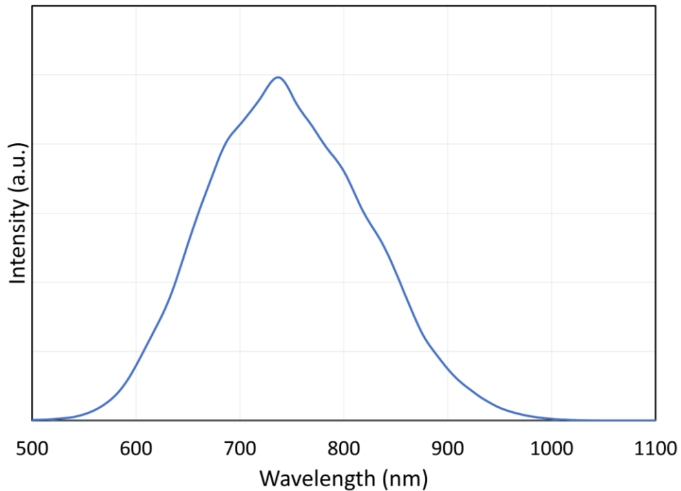
Figure 1: Photoluminescent emission spectra ( \lambda_{\text{exc}} = 365 \text{ nm} )
